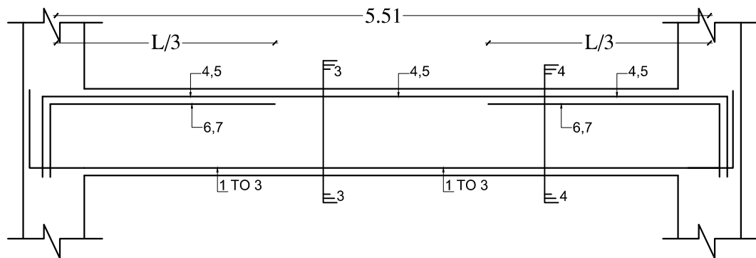
ROOF BEAM B-4
