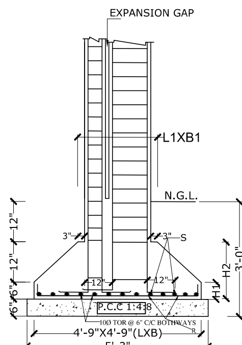
SECTION AT Y-Y
