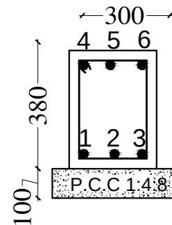
BEAM 'PB2'
