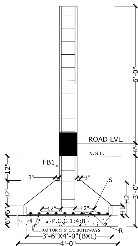
SECTION OF COLUMN AT B-B
