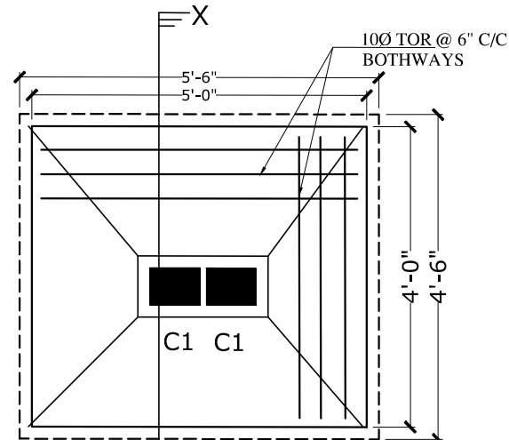
DETAIL OF FOUNDATION F2
