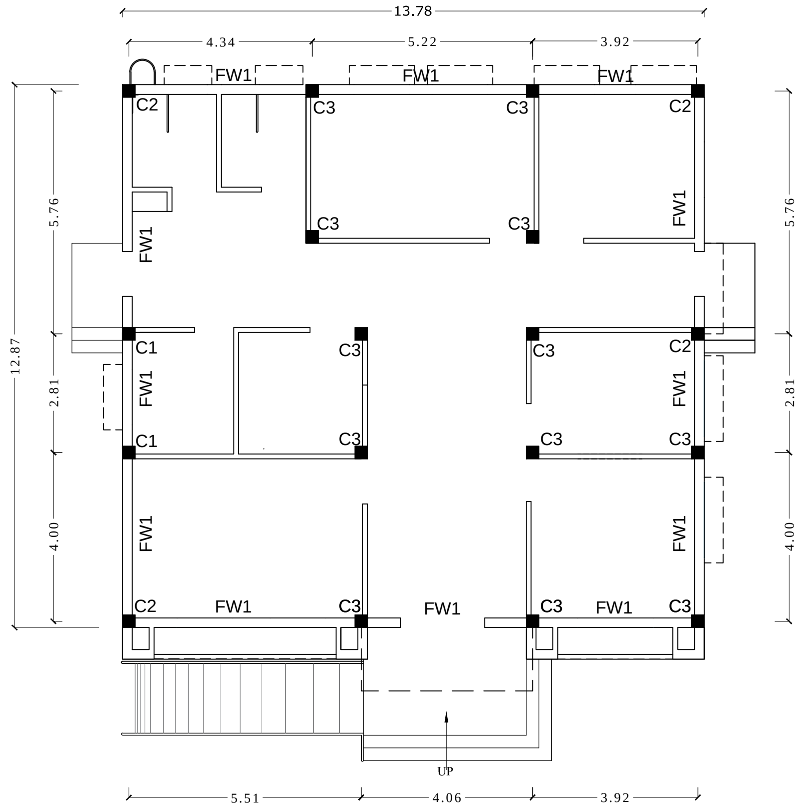
COLUMN LAYOUT PLAN
