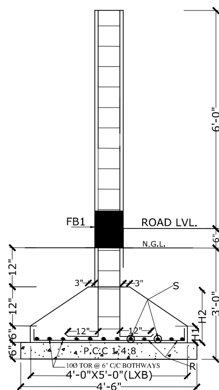
SECTION AT X-X
