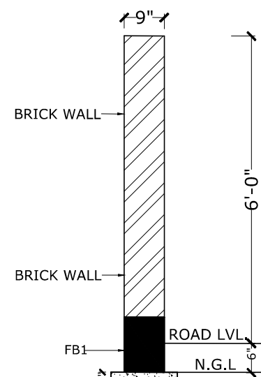
9" TH. BRICK WALL FOUNDATION. (SECTION AT 'A-A')
